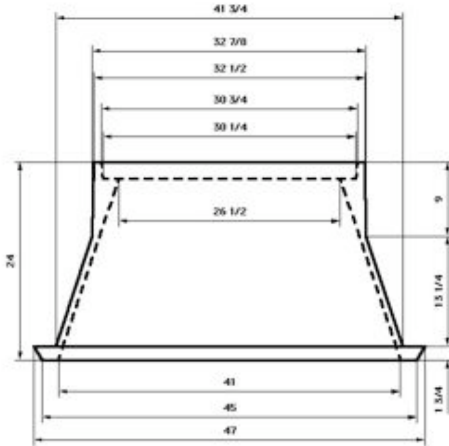
R264124-PCL Finished Casting Dimensional Drawing
